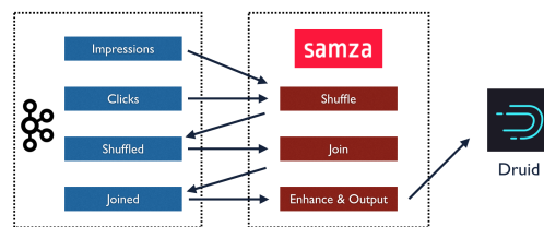
Figure 9: The streaming processing data pipeline.
