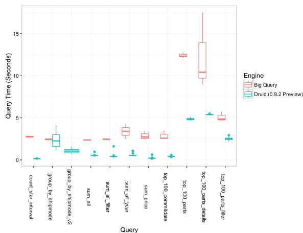
Figure 11: Druid benchmarked against Google BigQuery – 100GB TPC-H data.
