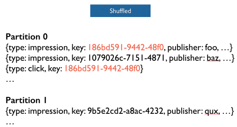
Figure 7: A shuffle operation ensures events to be joined at stored in the same Kafka partition.
