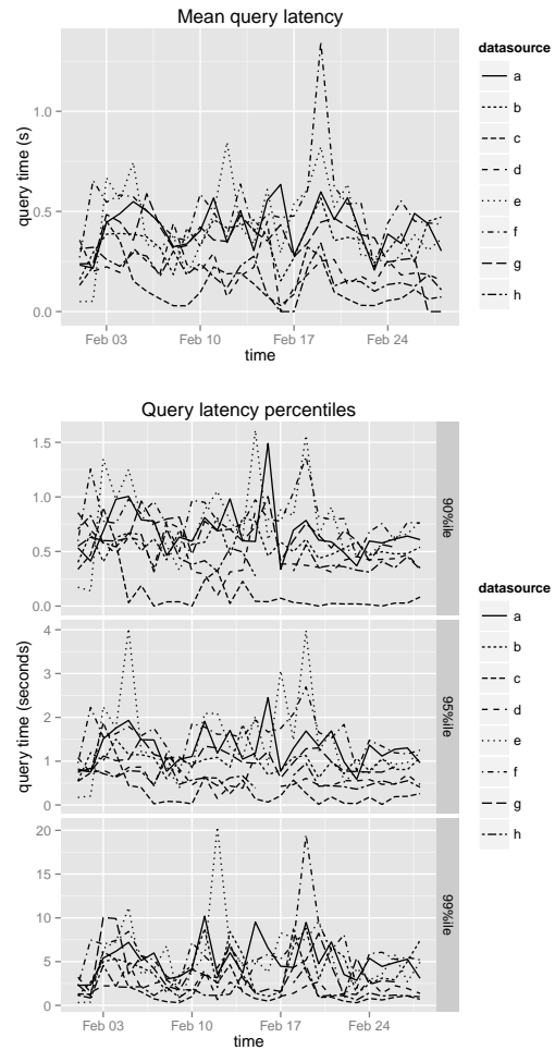
Figure 8: Query latencies of production data sources.
