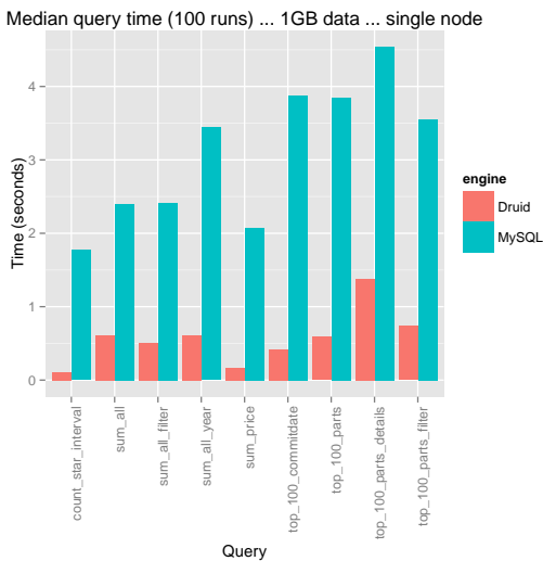
Figure 11: Druid and MySQL (MyISAM) benchmarks with the TPC-H 1 GB data set.
