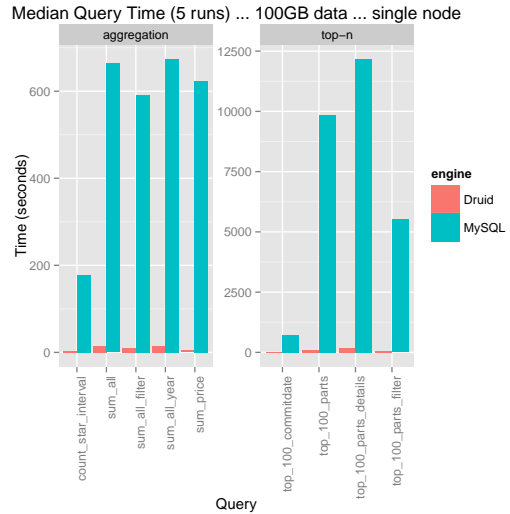
Figure 12: Druid and MySQL (MyISAM) benchmarks with the TPC-H 100 GB data set.
