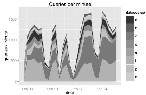
Figure 9: Druid production cluster queries per minute for multiple data sources.
