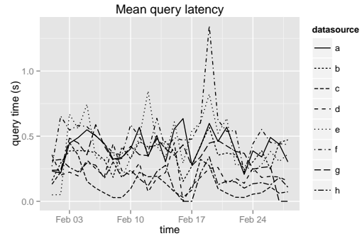
Figure 8: Druid production cluster average query latencies for multiple data sources.
