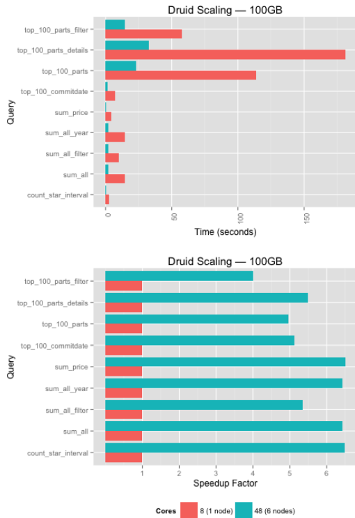
Figure 13: Scaling a Druid cluster with the TPC-H 100 GB data set.
