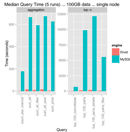
Figure 11: Druid & MySQL benchmarks – 100GB TPC-H data.
