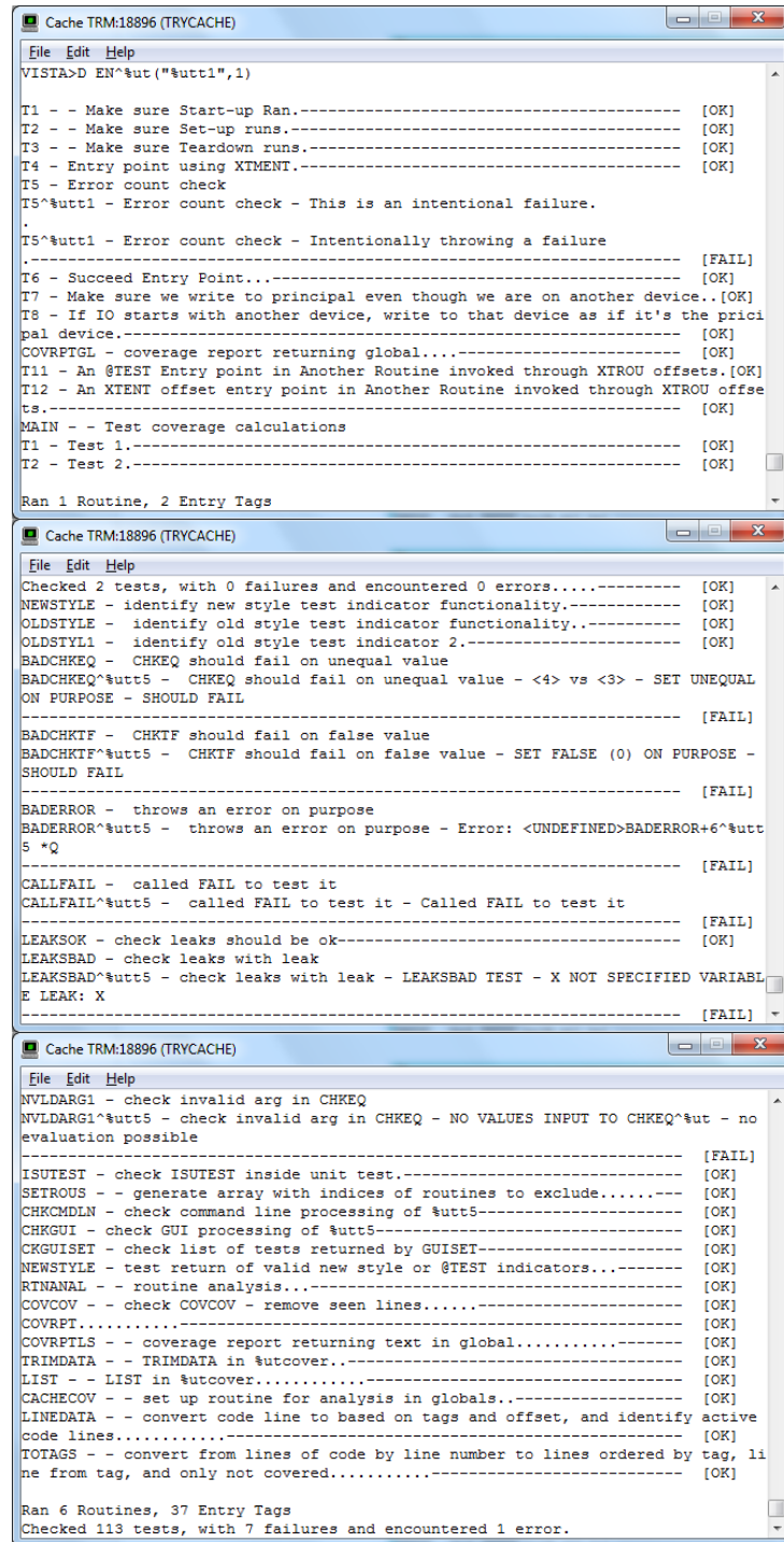
Figure 8. Command line unit tests for %utt1 with VERBOSE option
