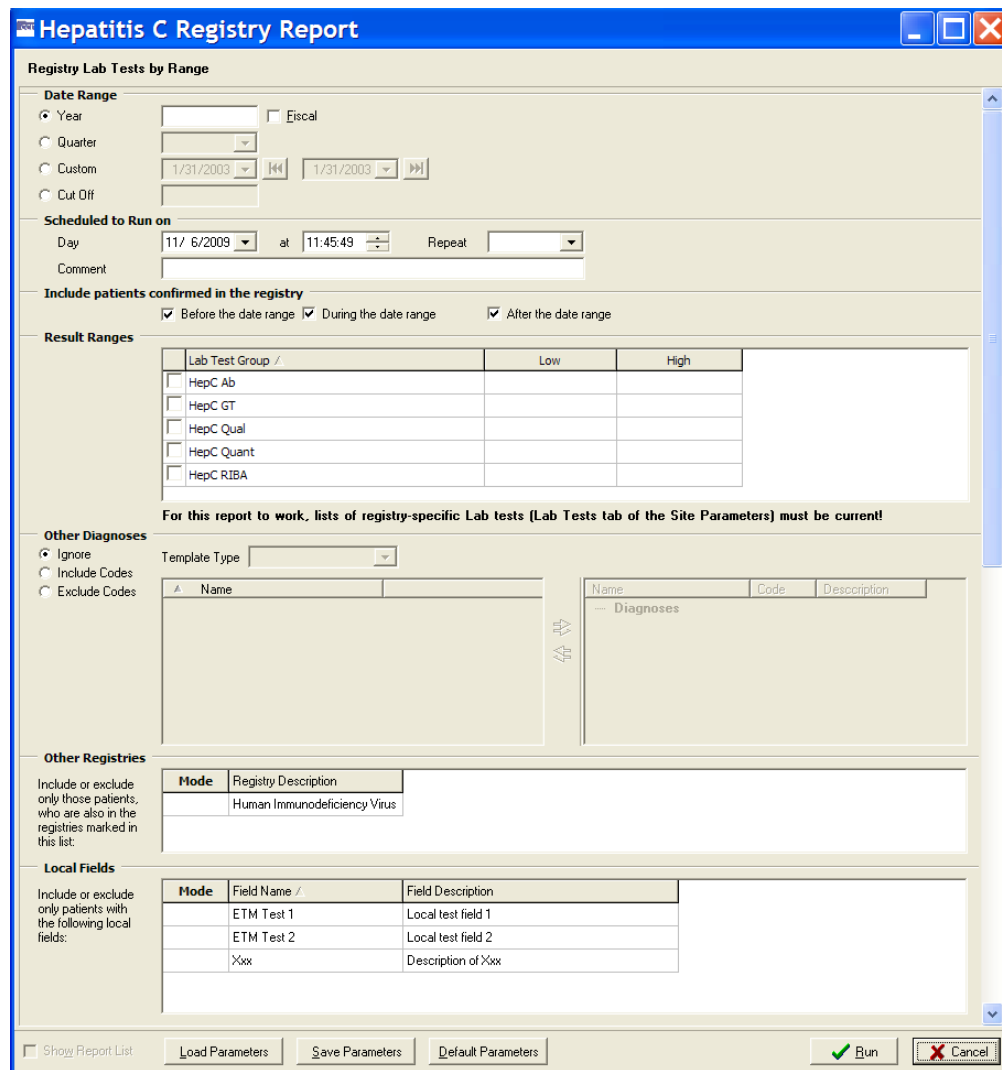
Figure 162 – Registry Lab Tests by Range Report Setup Screen
