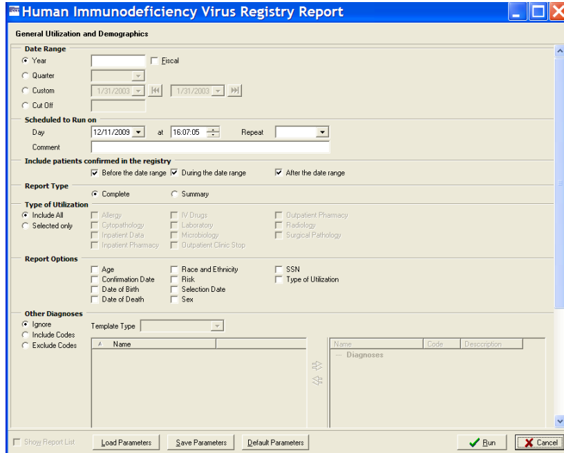
Figure 139 – General Utilization and Demographics Report Setup Screen
