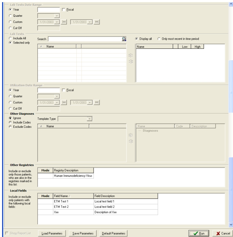
Figure 115 – Parts of the Report Setup Screen (2)
