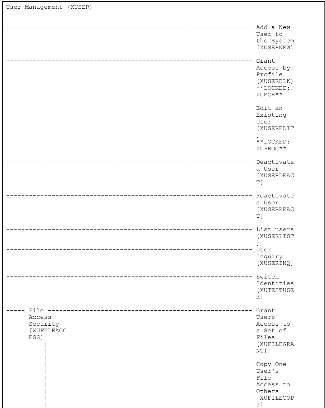
Figure 14. XUSER—Menu tree diagram
