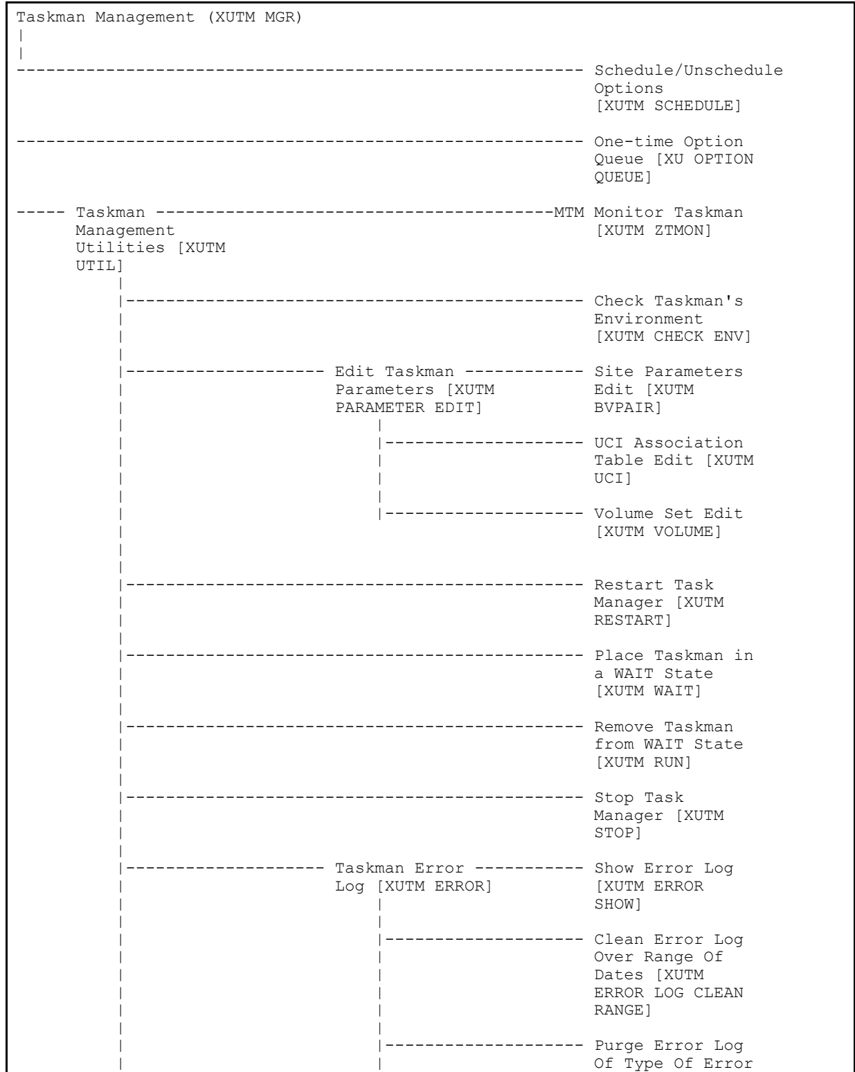
Figure 13. XUTM MGR—Menu tree diagram
