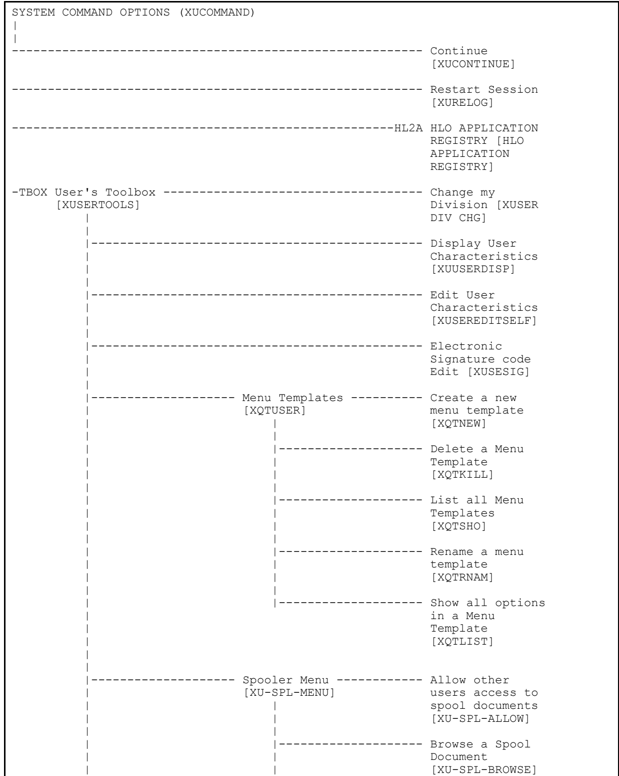
Figure 16. XUCOMMAND—Menu tree diagram
