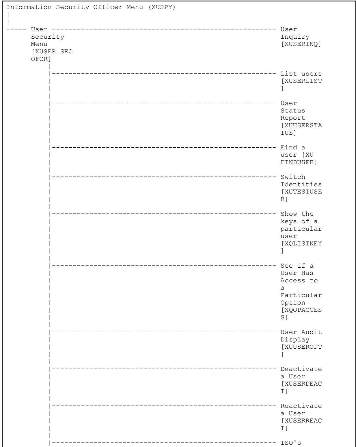
Figure 12. XUSPY—Menu tree diagram
