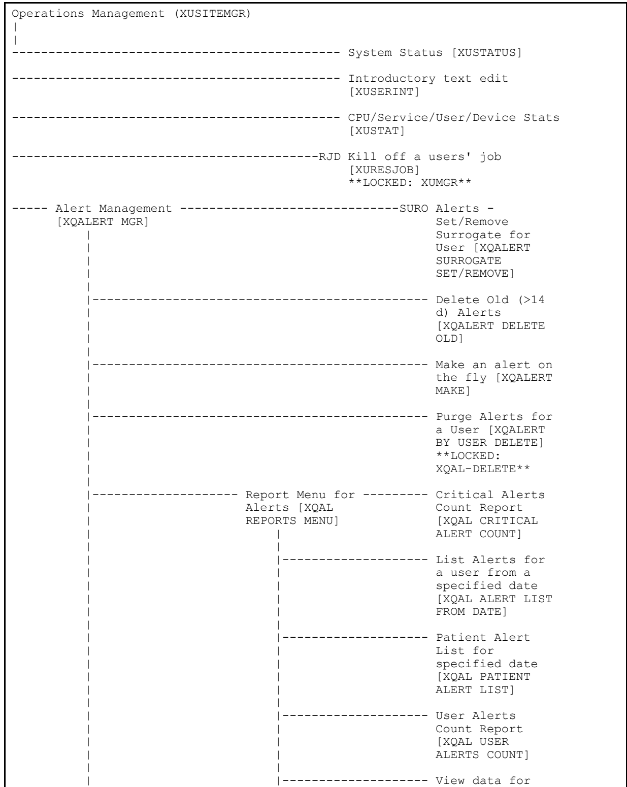
Figure 9. XUSITEMGR—Menu tree diagram
