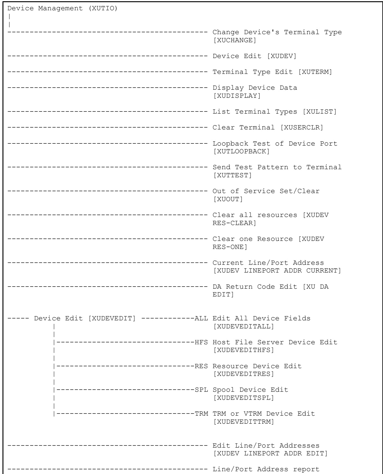
Figure 7. XUTIO—Menu tree diagram
