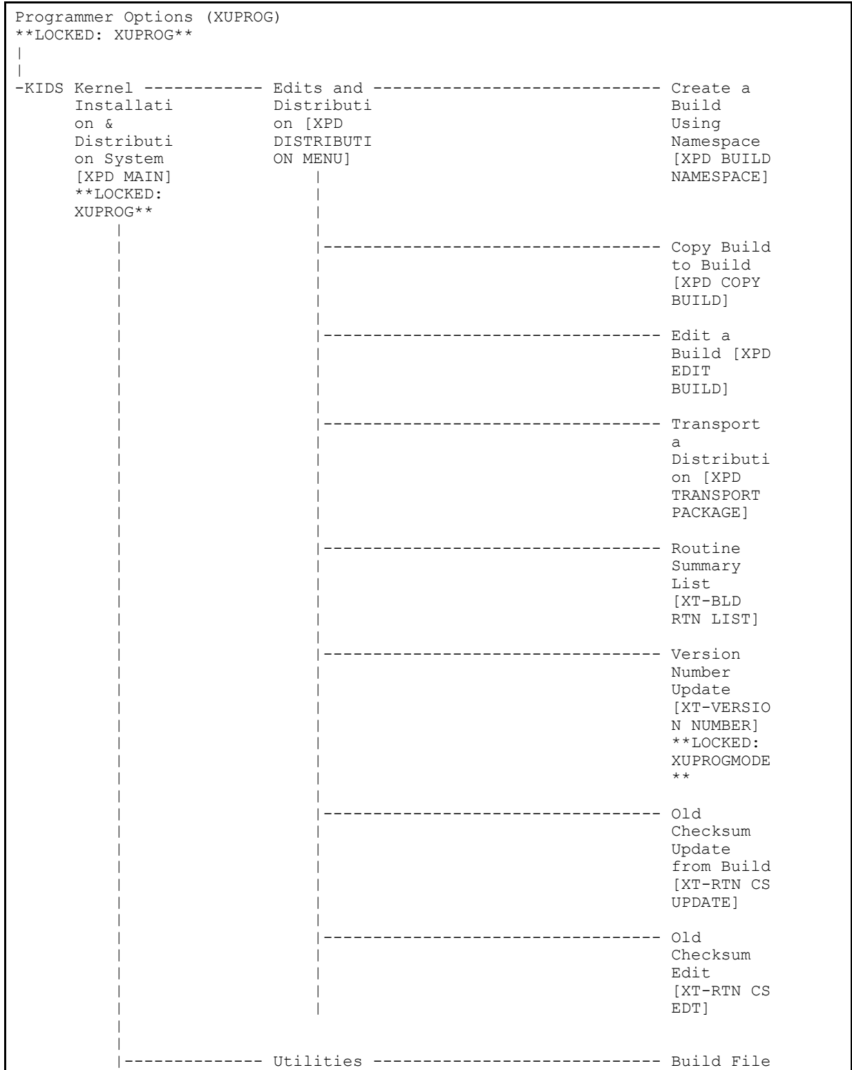
Figure 10. XUPROG—Menu tree diagram
