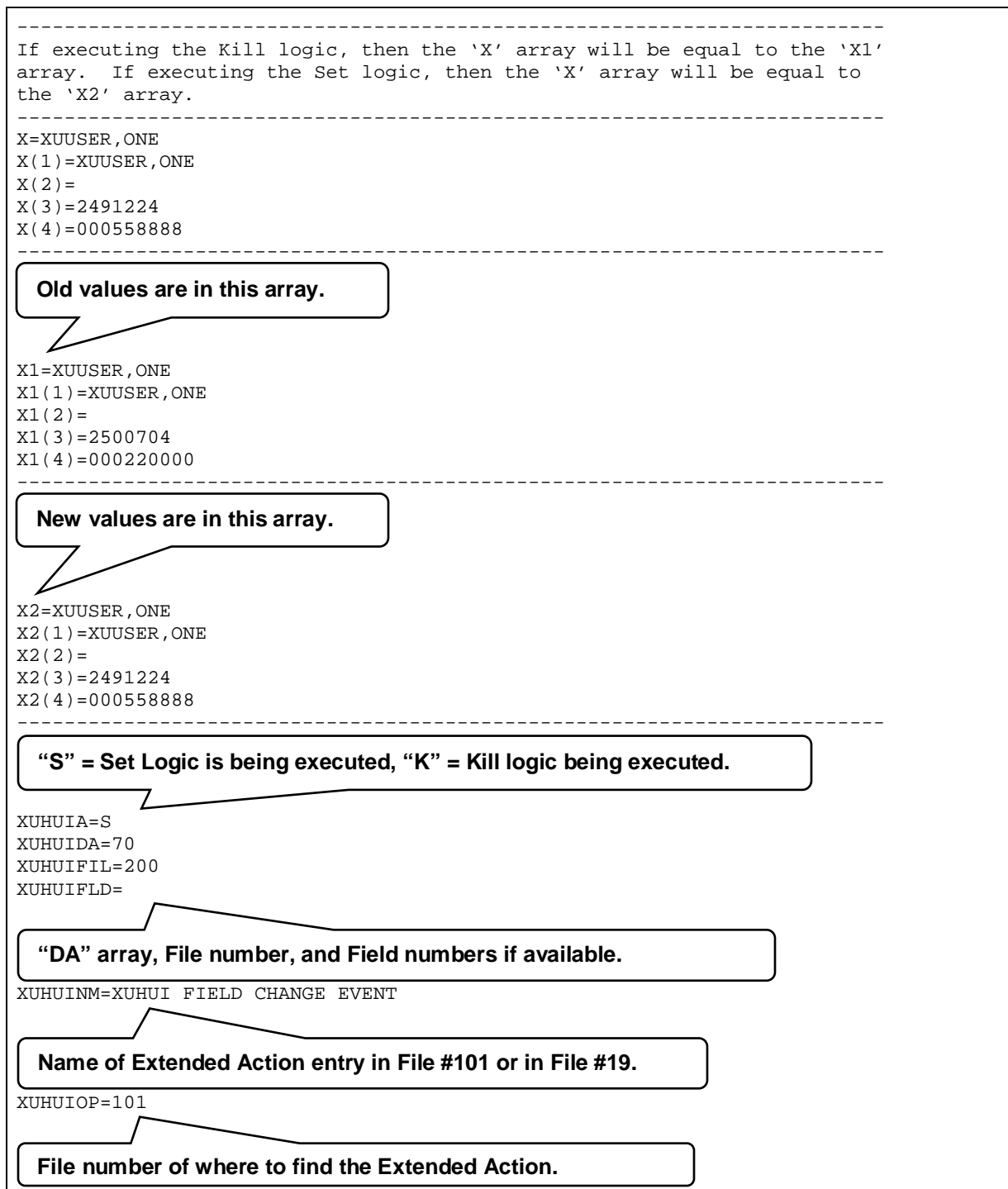
Figure 34. OPKG^XUHUI API—Example of internal results
