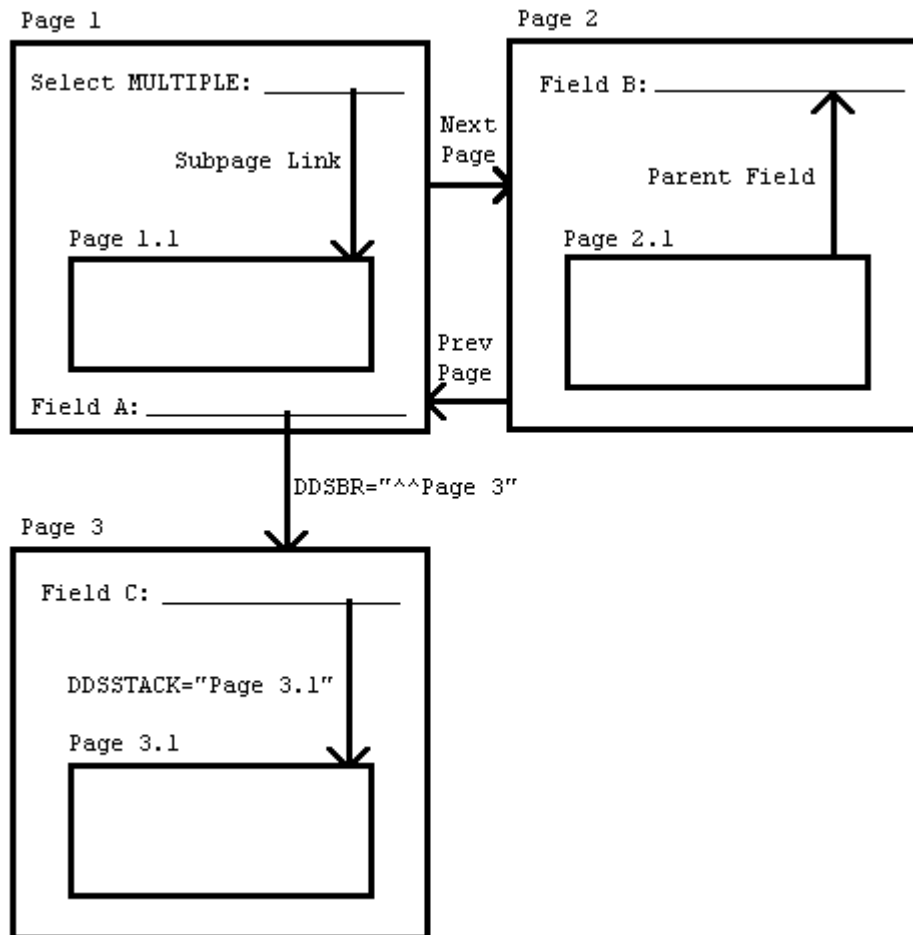
Figure 220. DDSSTACK variable—Sample page links
