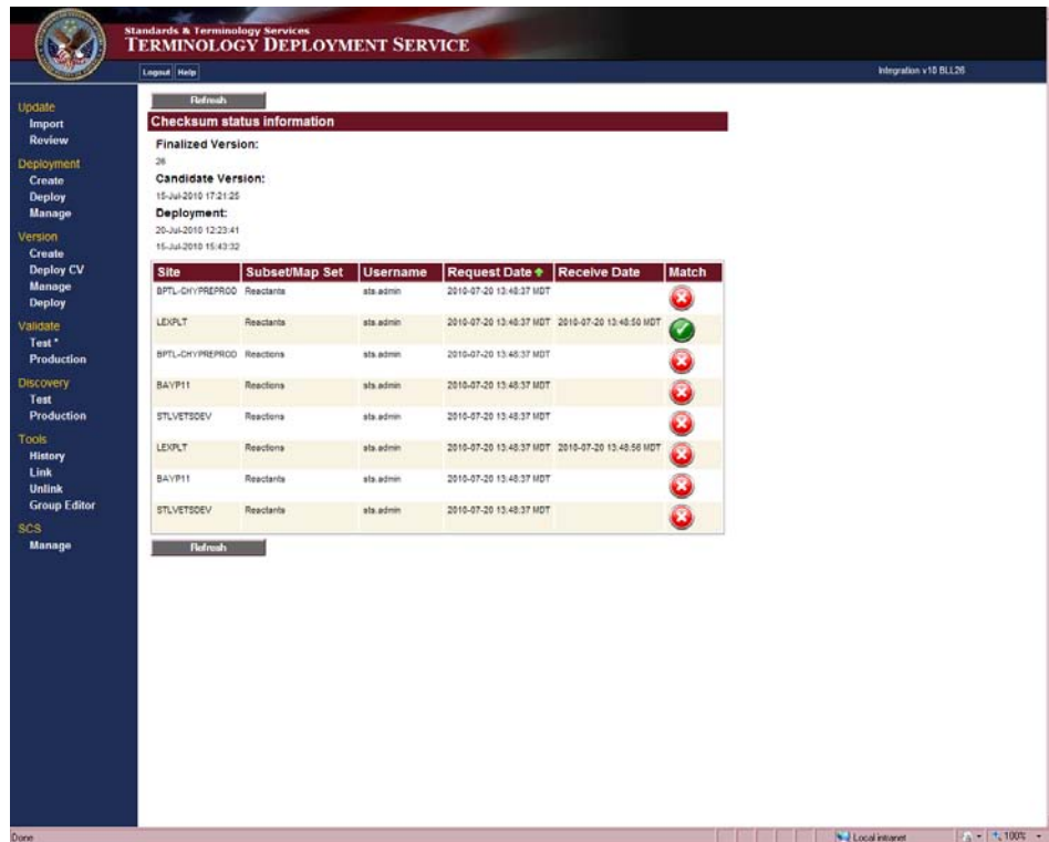
Figure 26. Display Checksum Results for Sites Window
