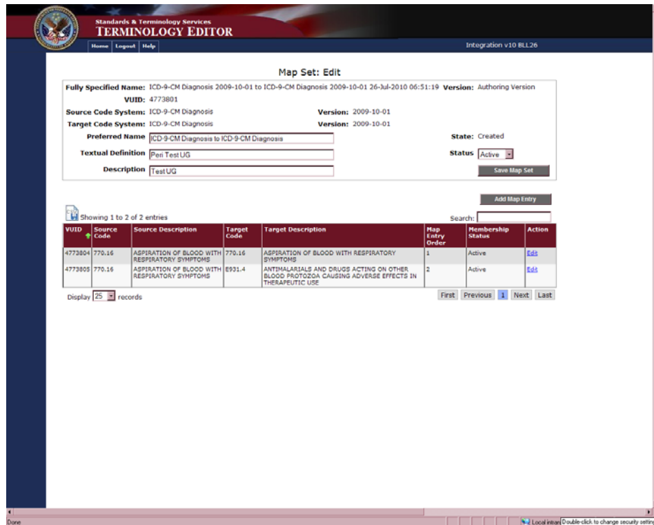
Figure 13. Map Set Edit Window
