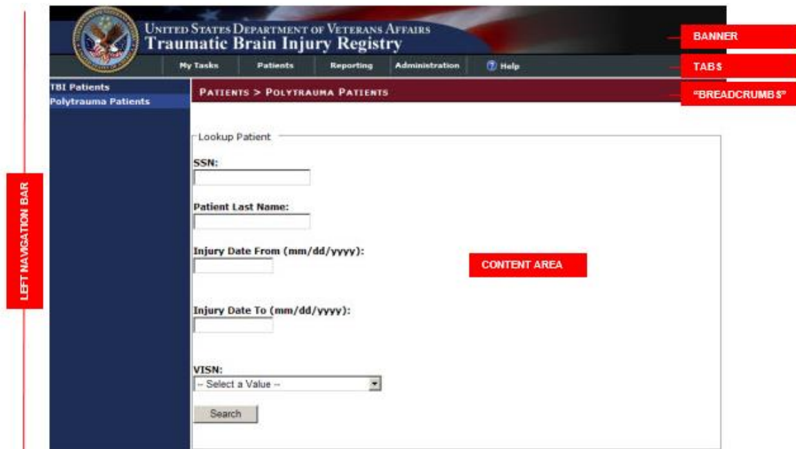
Figure 1 - Screen Areas
