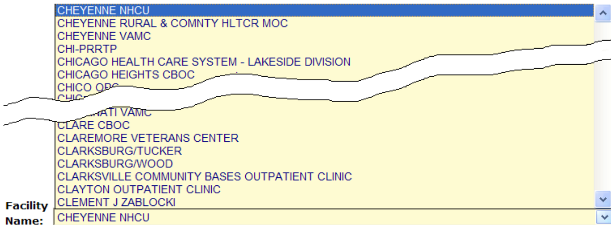
Figure 42 - Dropdown Sample 2
