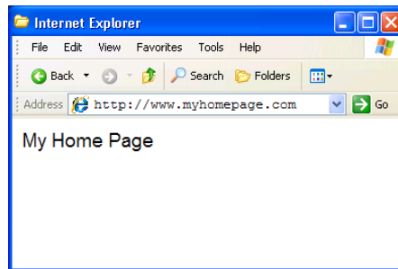
Figure 2 - Internet Explorer
