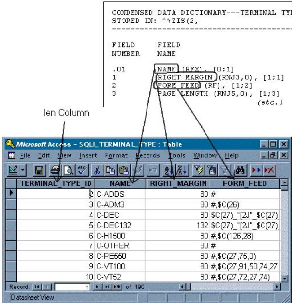
Figure 4-2: Projected column names for the SQLI_TERMINAL_TYPE table to the DD field names for the fields in the TERMINAL TYPE file (#3.2)
