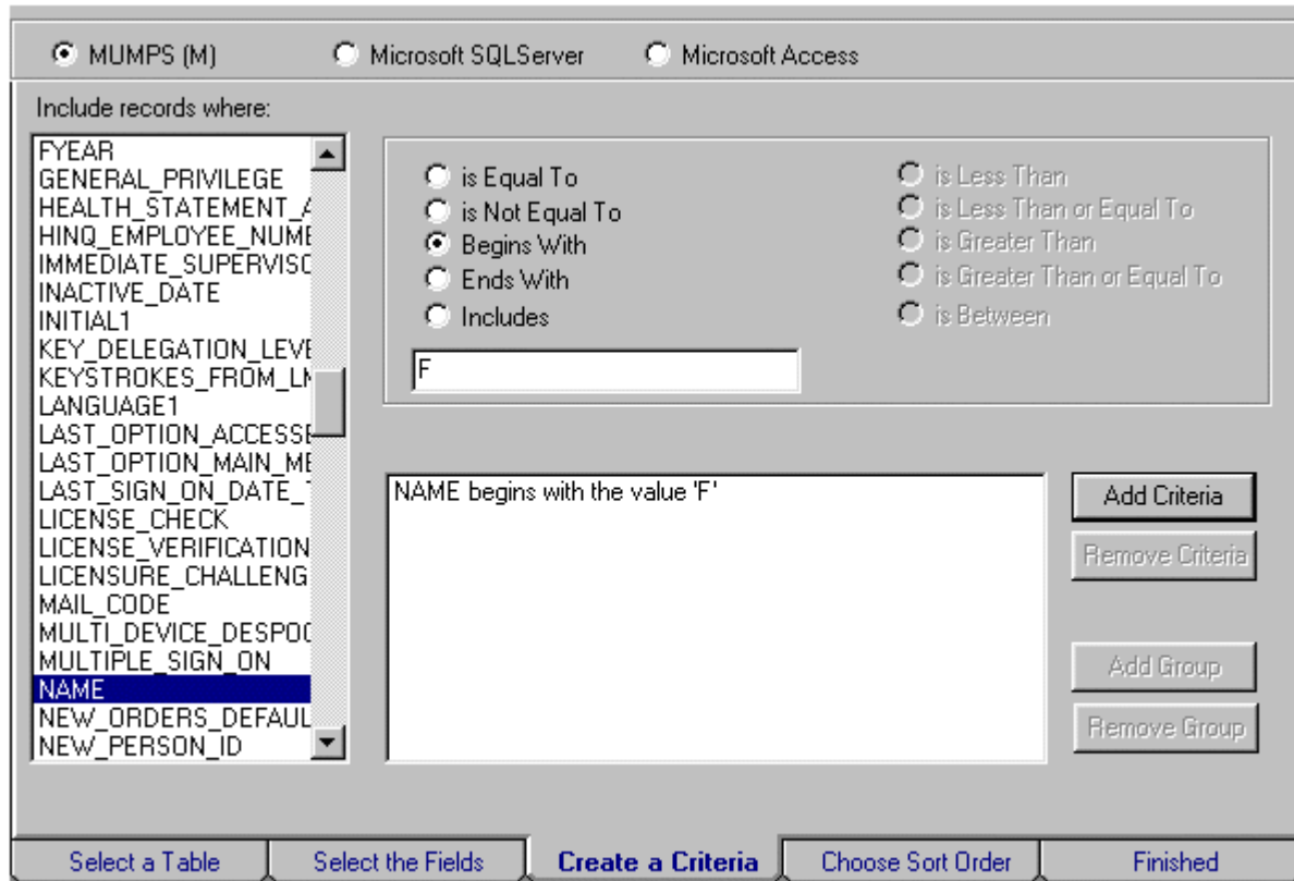
Figure 5-7: Step #3: Select Criteria—Names that begin with "F"
