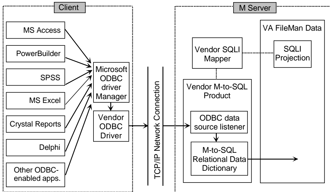
Figure 2-2: Sample system configuration (ODBC)
