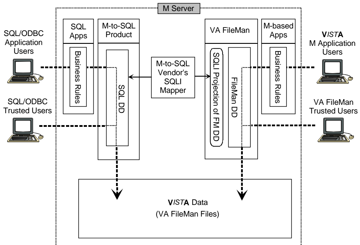
Figure 1-1: Relational view of VA FileMan
