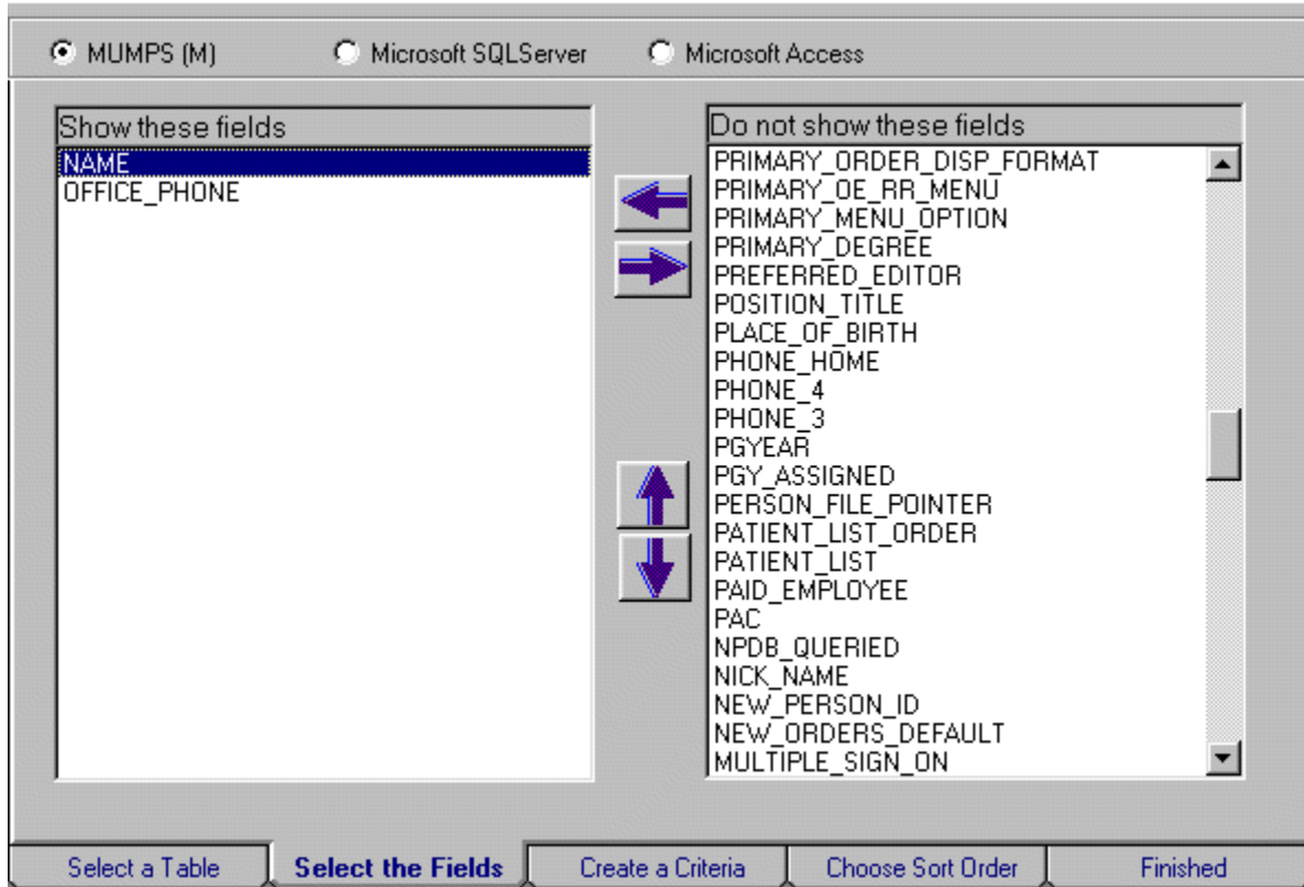
Figure 5-6: Step #2: Select the fields
