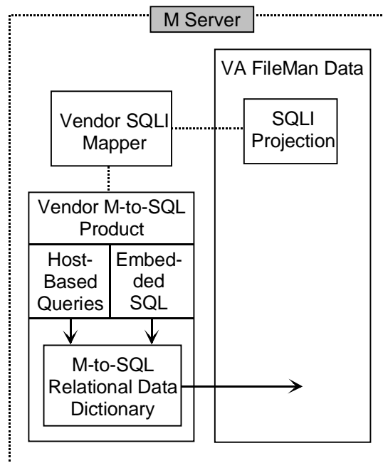
Figure 2-1: Sample system configuration (host-based queries)
