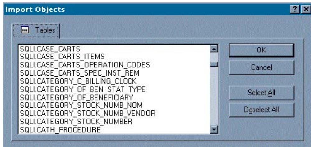
Figure 4-1: Partial list of SQLI table names for VA FileMan top-level files and subfiles
