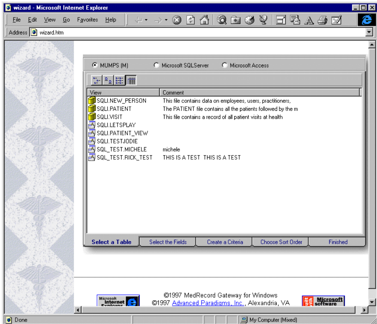
Figure 5-5: Step #1: Select tables or view
