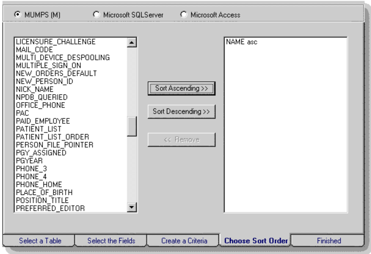
Figure 5-8: Step #4: Choose sort order
