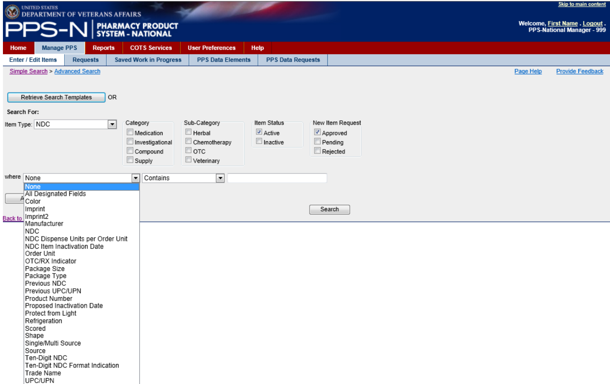
Figure 21: Advanced Search Dropdown List
