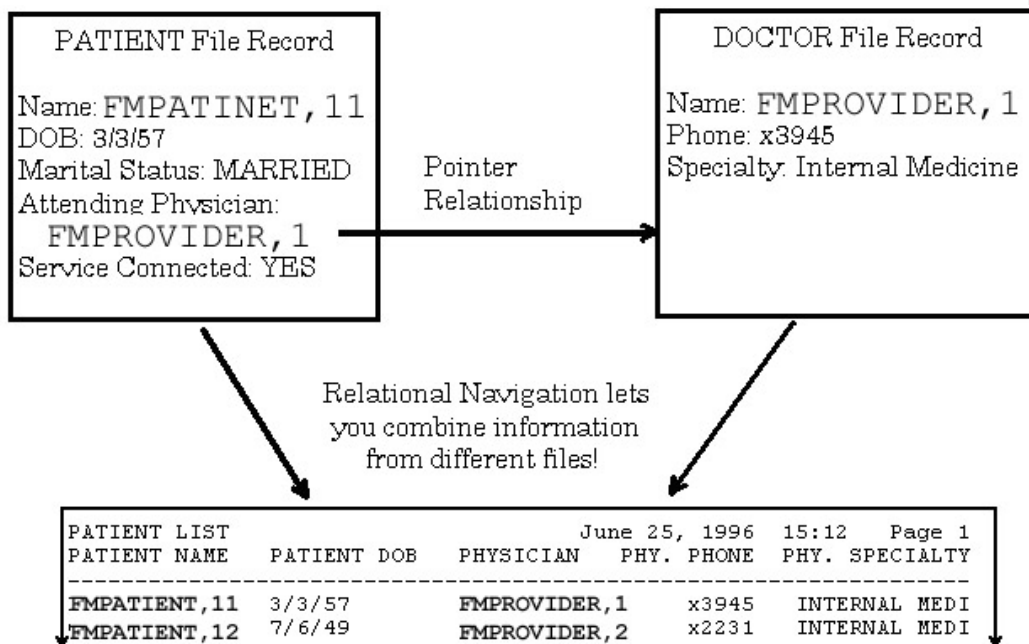
Figure 34: Relational Navigation—Example illustrating relational navigation
