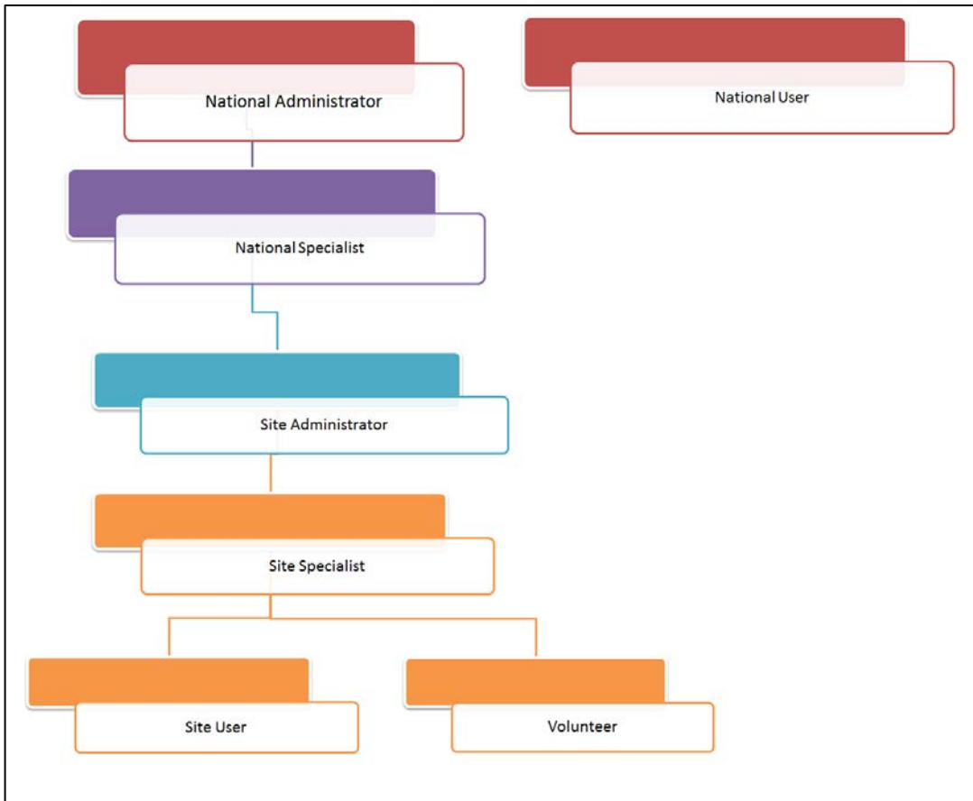
Figure 20 - Permission Hierarchy
