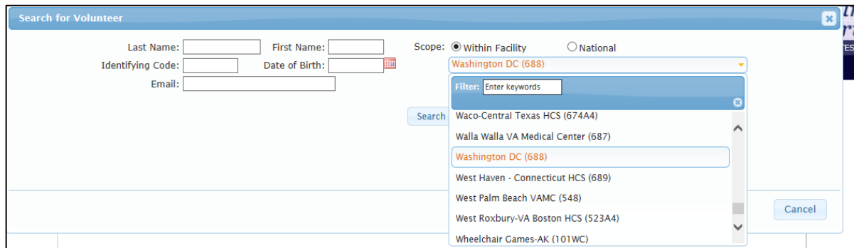
Figure 4 - Dropdown Menu
