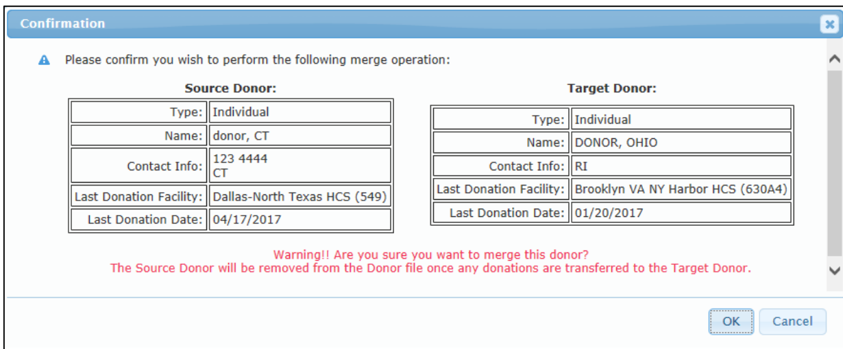
Figure 112 - Merging Donor
