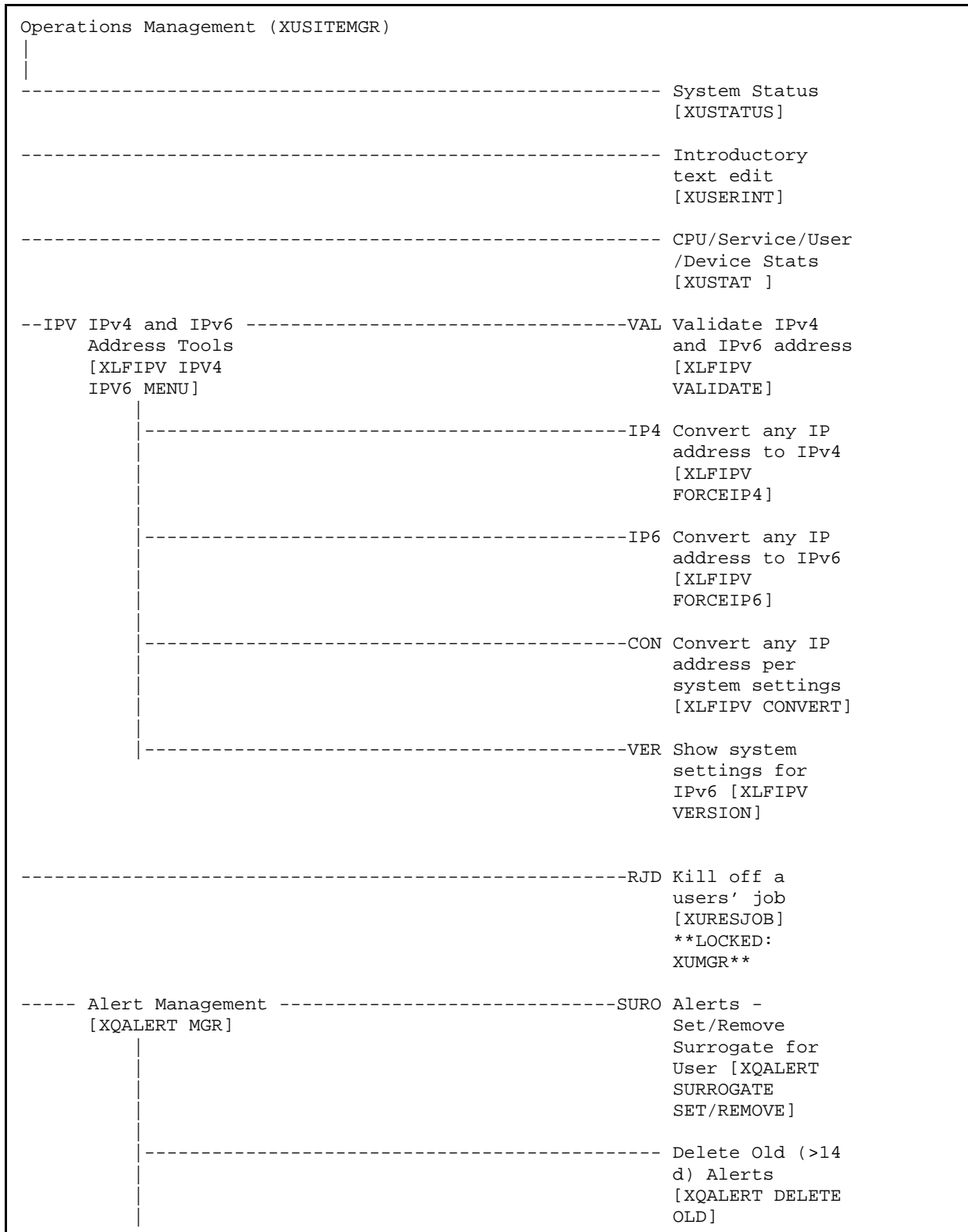
Figure 9: XUSITEMGR—Menu Tree Diagram: Sample from OAKTST “Gold” Account
