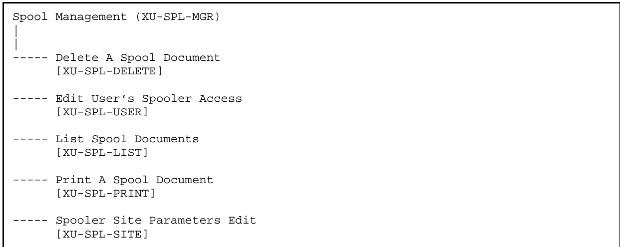
Figure 11: XU-SPL-MGR—Menu Tree Diagram: Sample from OAKTST “Gold” Account
