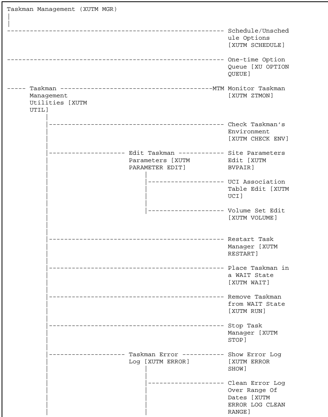
Figure 13: XUTM MGR—Menu Tree Diagram: Sample from OAKTST “Gold” Account
