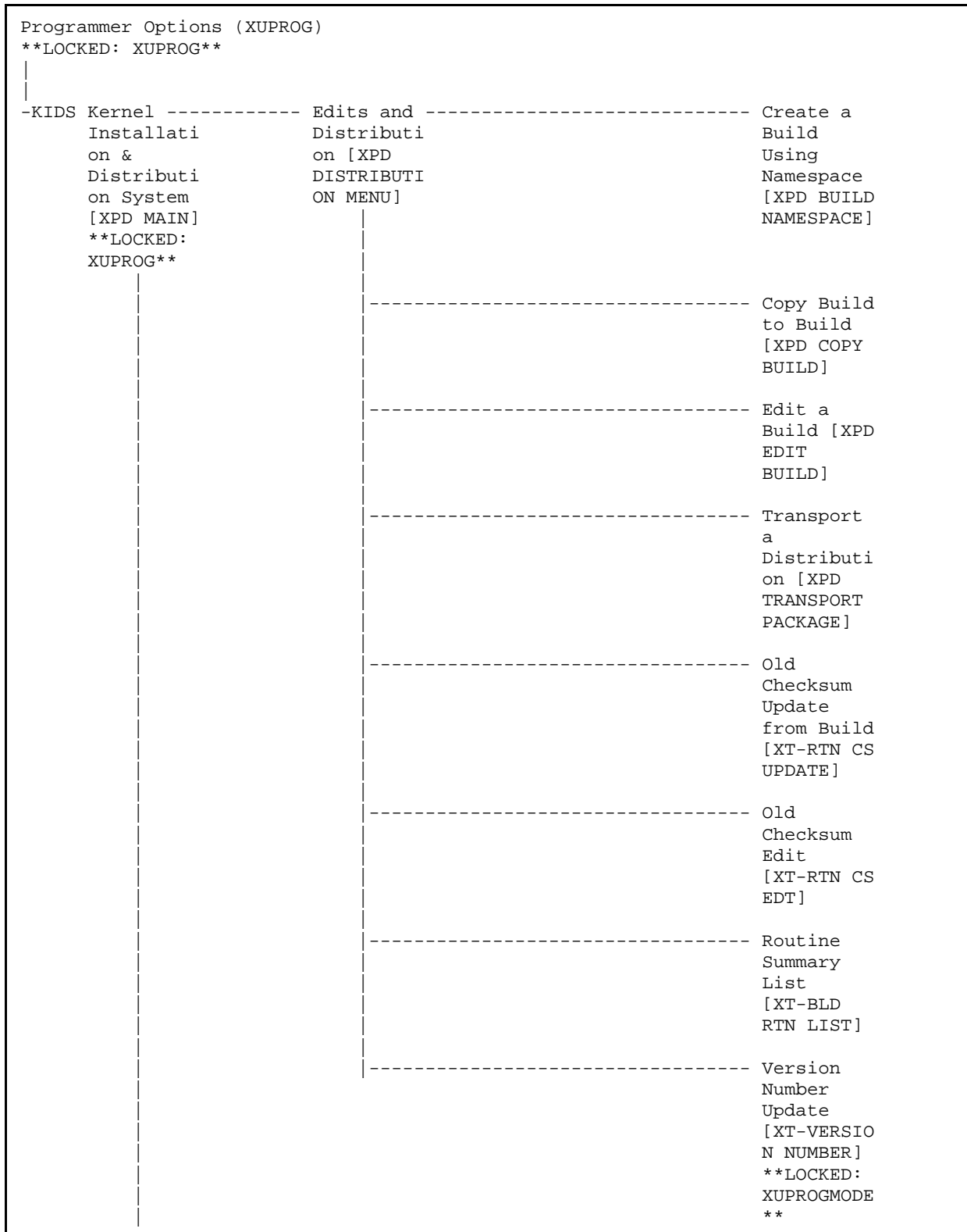
Figure 10: XUPROG—Menu Tree Diagram: Sample from OAKTST “Gold” Account
