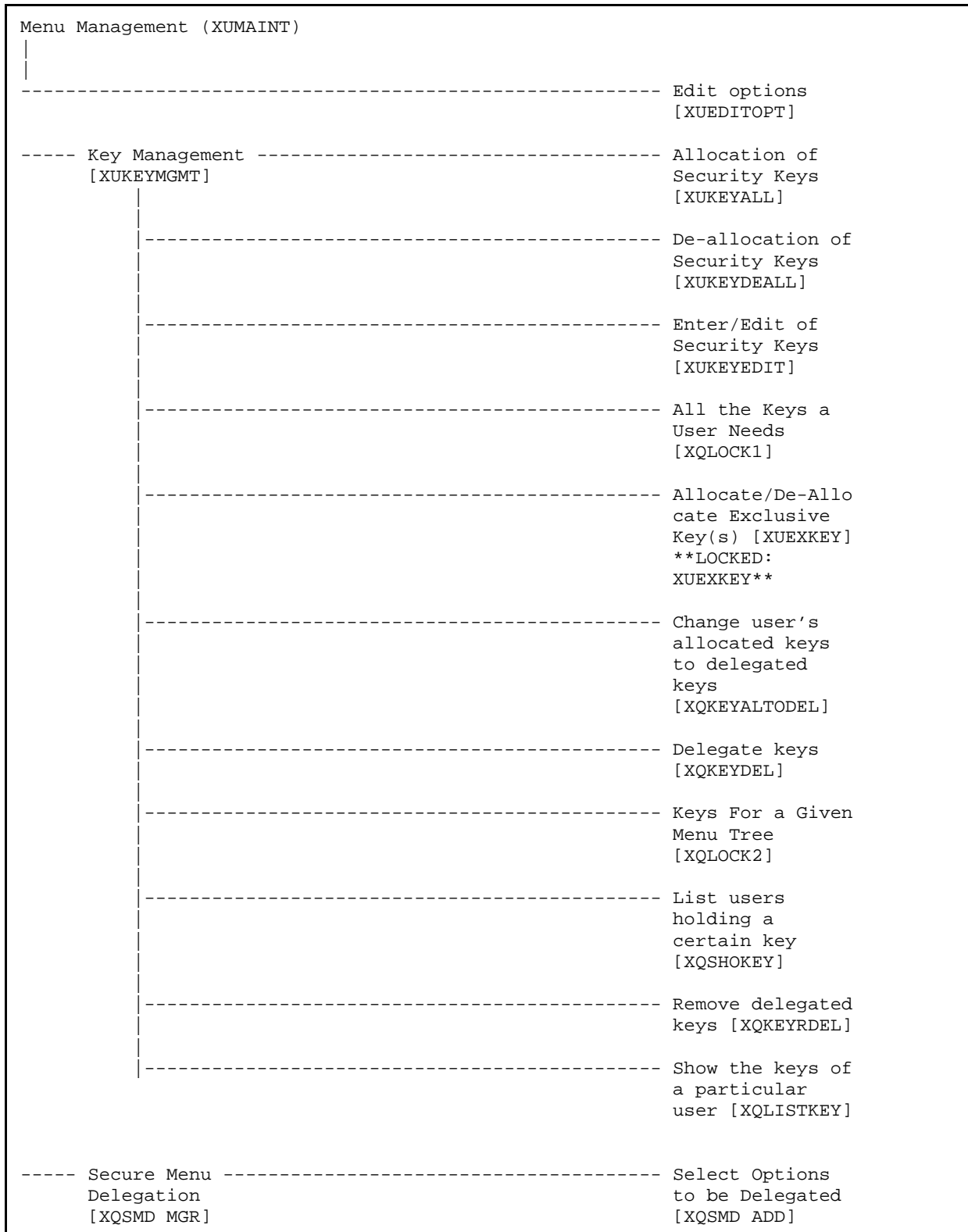
Figure 8: XUMAIN—Menu Tree Diagram: Sample from OAKTST “Gold” Account
