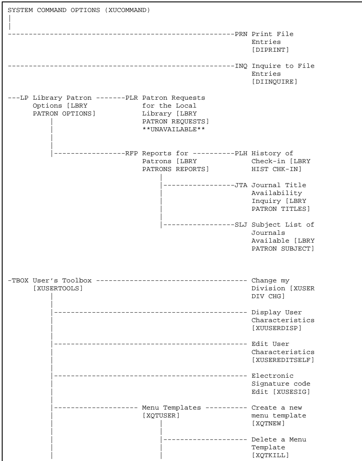
Figure 16: XUCOMMAND—Menu Tree Diagram: Sample from OAKTST “Gold” Account
