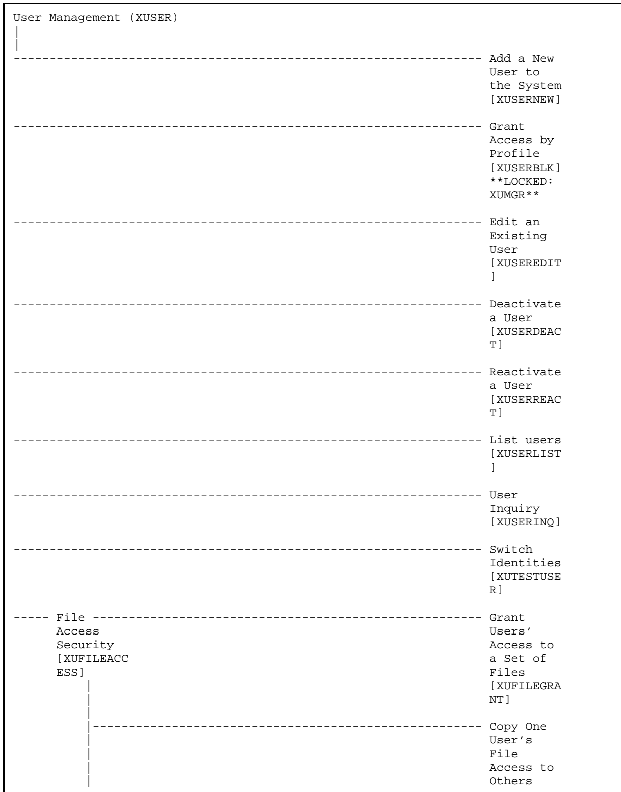
Figure 14: XUSER—Menu Tree Diagram: Sample from OAKTST “Gold” Account
