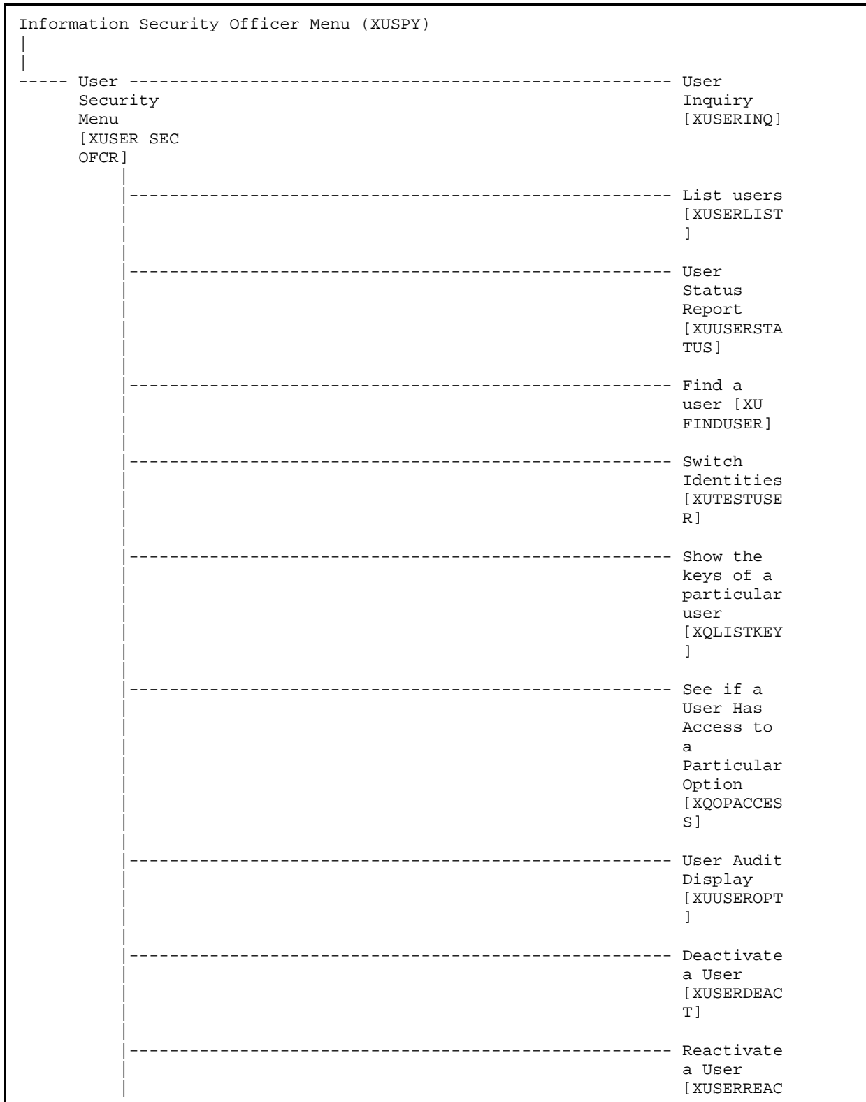
Figure 12: XUSPY—Menu Tree Diagram: Sample from OAKTST “Gold” Account
