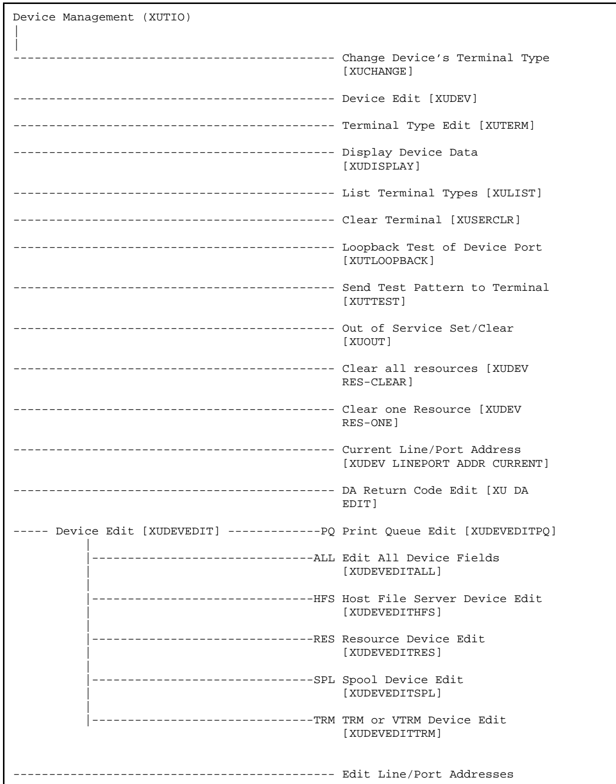
Figure 7: XUTIO—Menu Tree Diagram: Sample from OAKTST “Gold” Account
