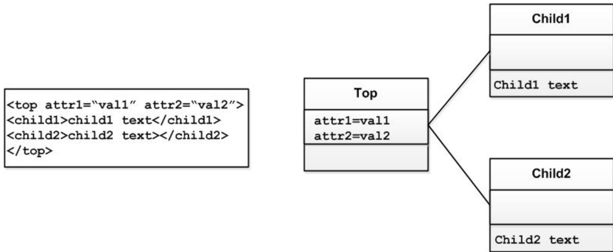
Figure 513: XML Document (left)—Tree Structure Diagram (right)
