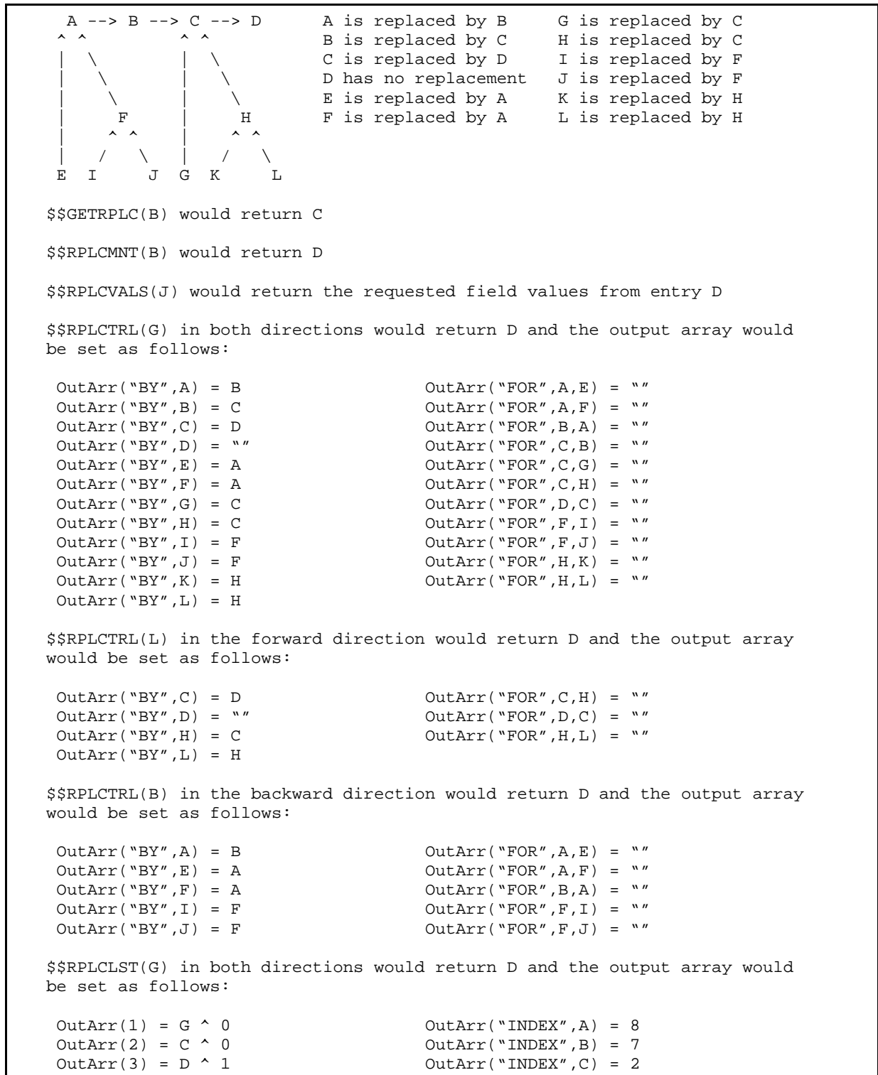
Figure 222: Toolkit—Replacement Relationships: Data Standardization
