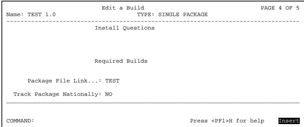
Figure 117: KIDS—Screen 4 of Edit a Build Sample
