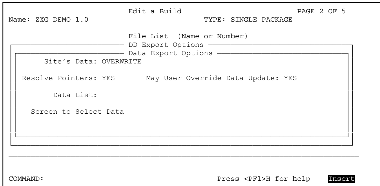
Figure 104: KIDS—Settings for Sending Data
