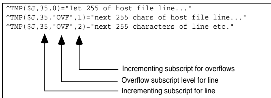
Figure 74: Host Files—Overflow Lines in a Host File Sample
