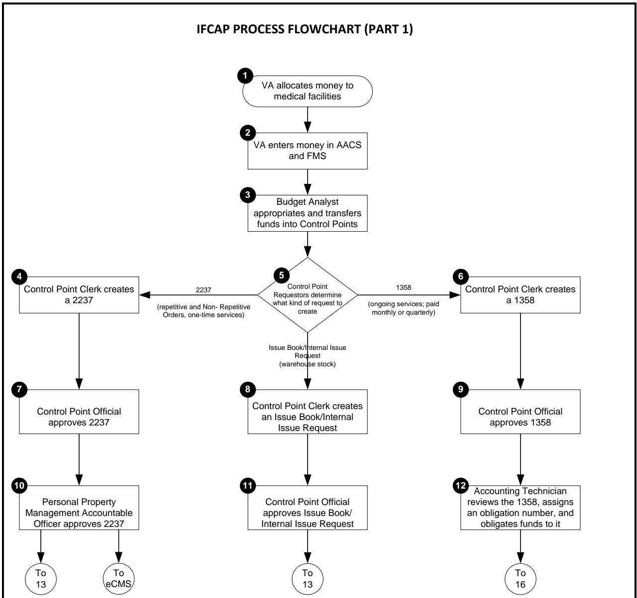
Figure 9-3. IFCAP Process Flowchart (Part 1)
