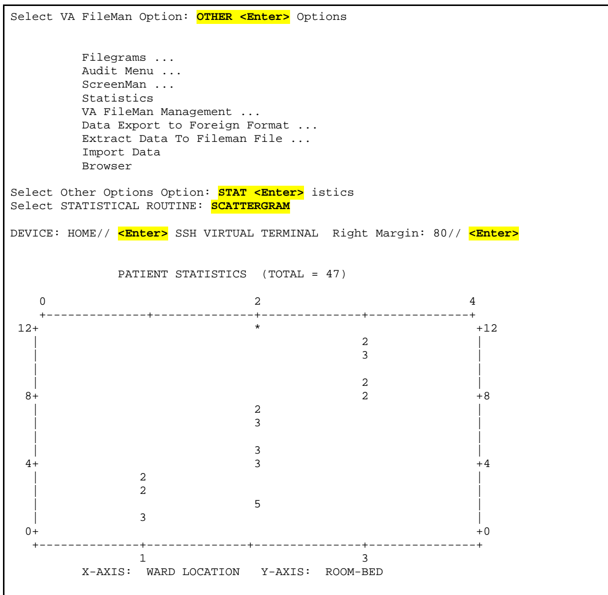
Figure 87: Statistics—Generating dialogue and sample output of a Scattergram
