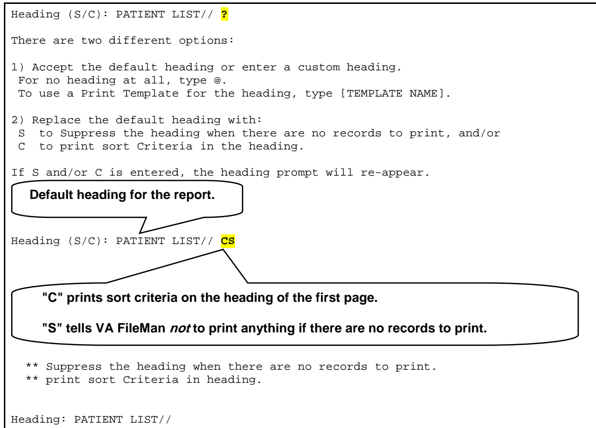
Figure 32: Print—Dialogue to customize report headings: Sample user entries at prompts
