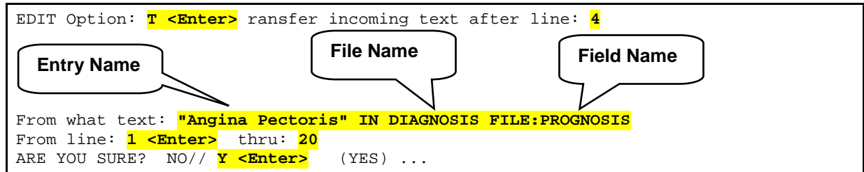
Figure 119: Line Editor—Dialogue of the Extended Pointer Syntax while using the Transfer Lines From Another Document option: Sample user entries at prompts (Example #2)
