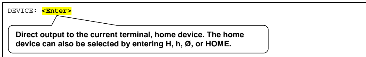
Figure 147: Choosing the Home Device
