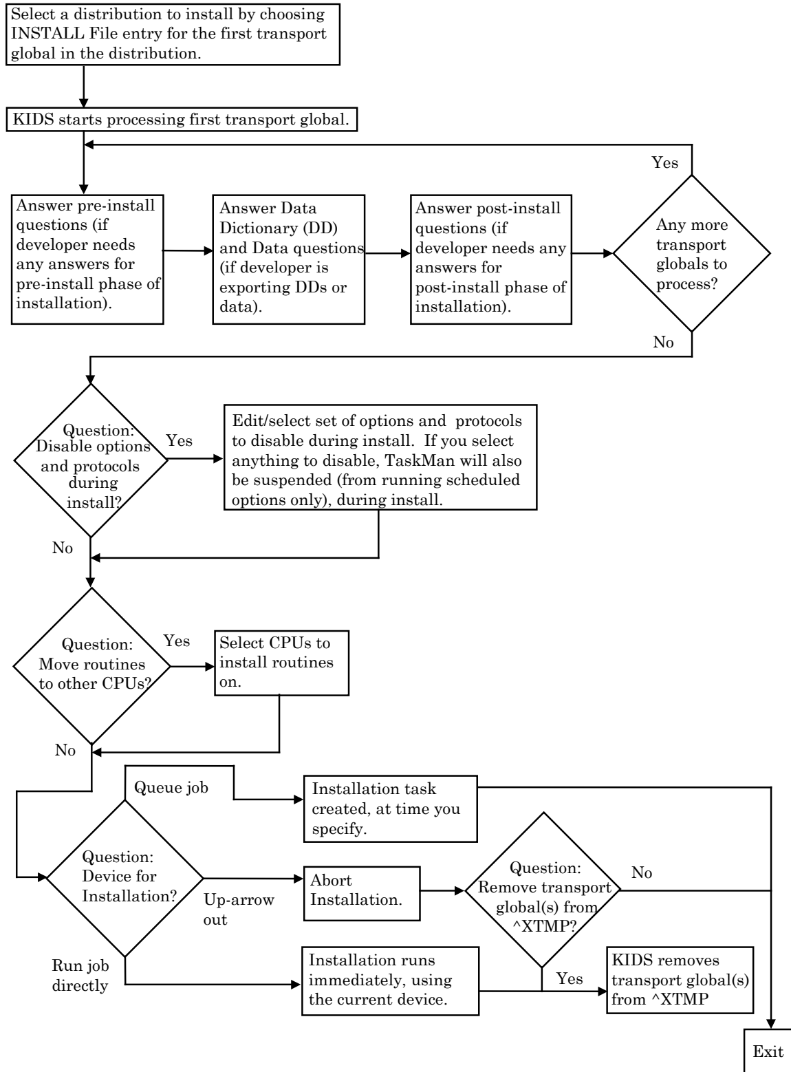
Figure 292: Answering Installation Questions for a Distribution—Flowchart
