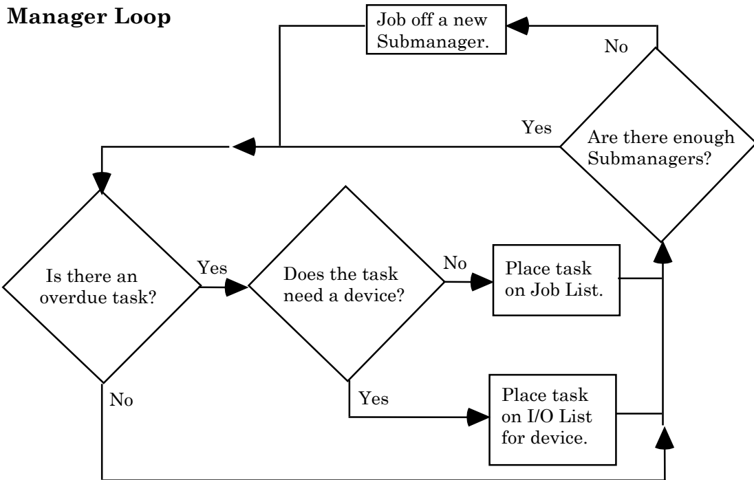
Figure 231: TaskMan Manager and Submanager Process Flow Diagram
